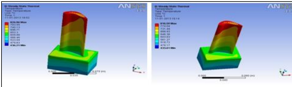
Fig 7. Temperature distribution for 13holes Fig 8. Temperature distribution for 13holes
