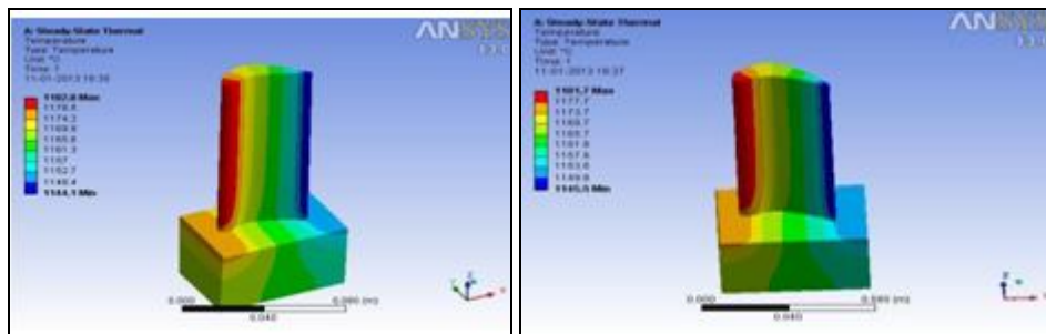
Fig 1. Temperature distribution for solid(N155) Fig 2. Temp distribution for solid(Inconel718)
