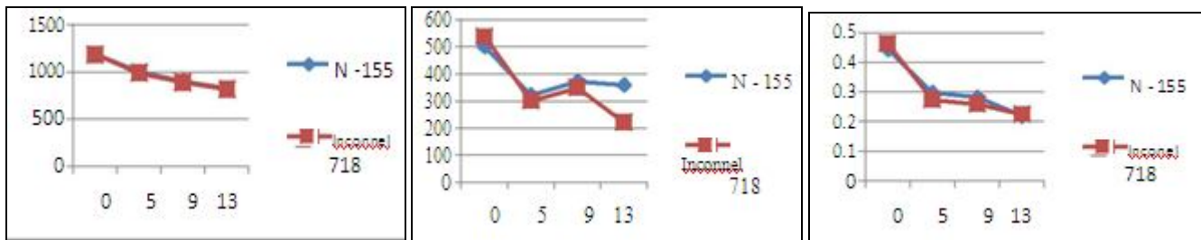
Fig 13 .Max. Temperature Vs. No of holes
