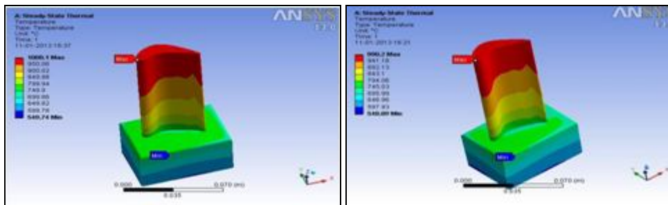
Fig 3. Temp. Distribution for 5 holes(N - 155) Fig 4. Temp. distribution for 5holes (Inconel 718)
