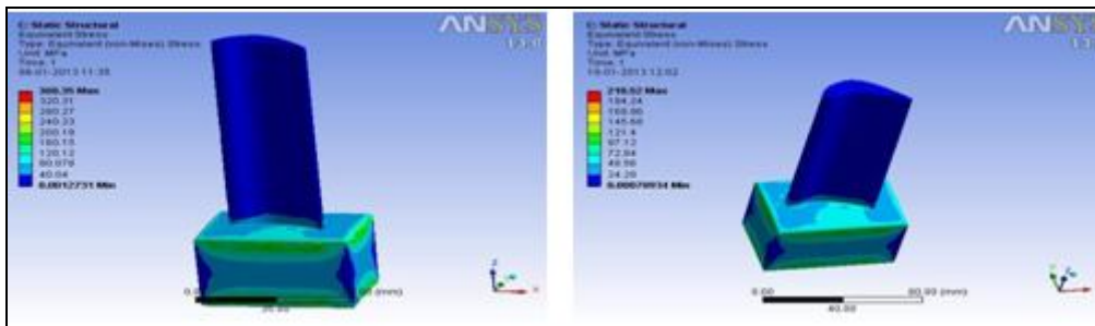
Fig 11. Stress distribution for 13 holes Fig 12. Stress distribution for 13 holes
