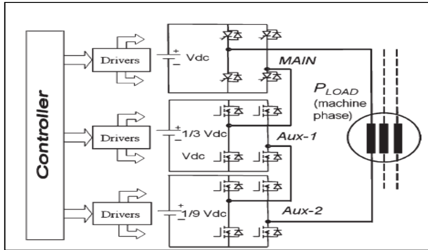
Figure 4: Main Components Of 27 Level Asymmetrical Type Multi Level Inverter For 1 Phase
