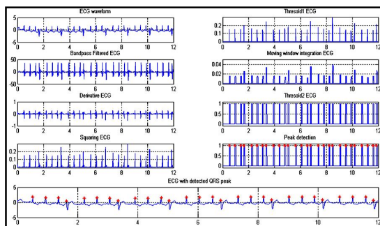
Figure 1.15: QRS peak detection Algorithm/structure processing steps for Second degree AV Block
