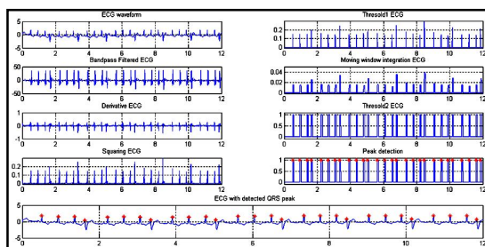
Figure 1.14: QRS peak detection Algorithm/structure processing steps for Tachycardia
